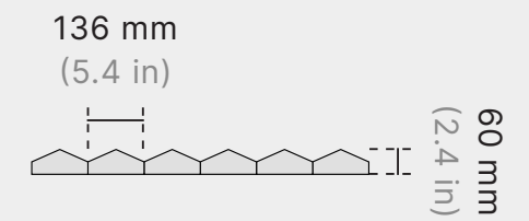
Caret Detail
